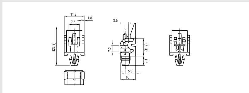
PWB side t=1.6±0.15 chassis side t=0.8~2.3
